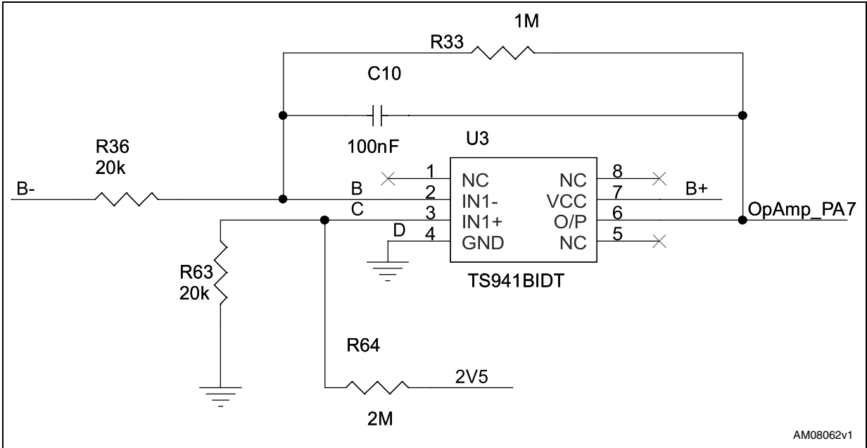
Figure 9. OP-AMP-section
