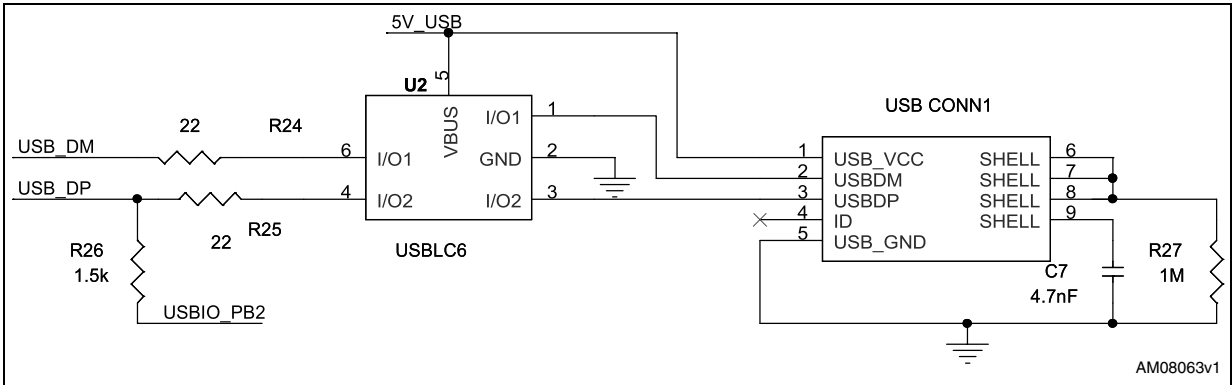
Figure 10. USB section
