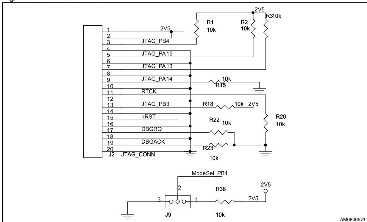
Figure 12. JTAG-CONN section
